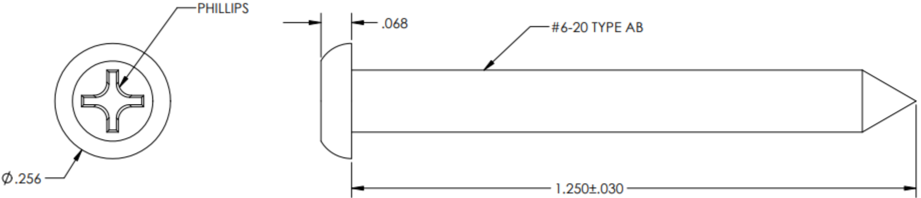
Trim Ring Mounting Screw
