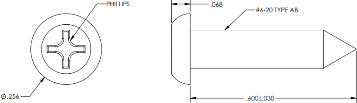
Plastic Door Locking Screw
