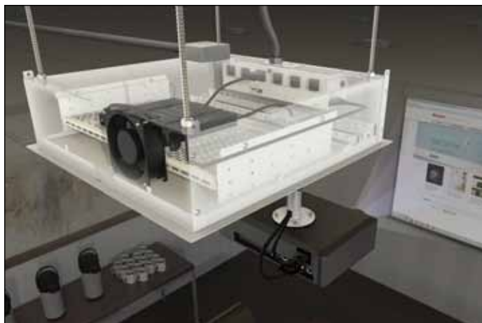
Evolution Series controlled receptacle ceiling box with projector mount (ECB2SP-CR) installed in a conference room.
