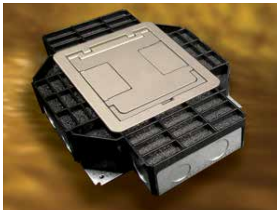
RFB2-0G Floor Box with FloorPort Cover
