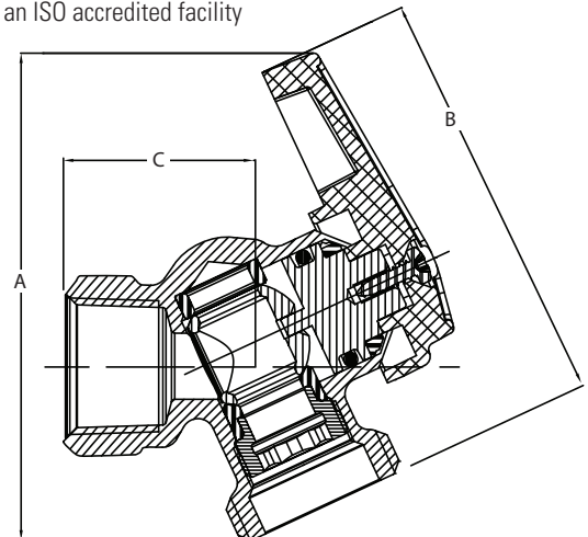
Pictured R-672NL Cut-away
