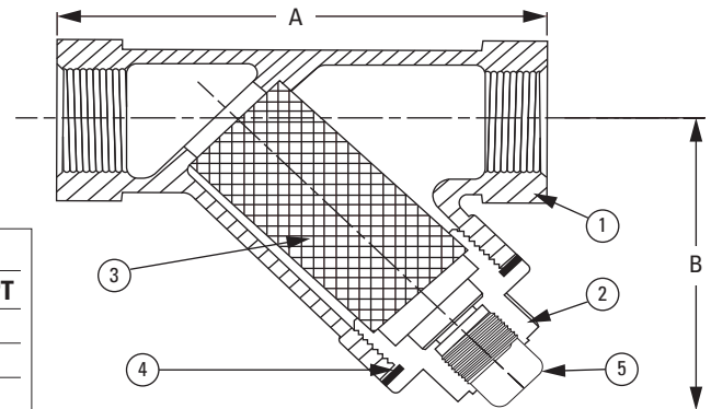
Pictured: T/S-15NL Cut-away view
