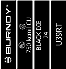
BARREL MARKING
