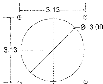
MOUNTING DIMENSIONS
