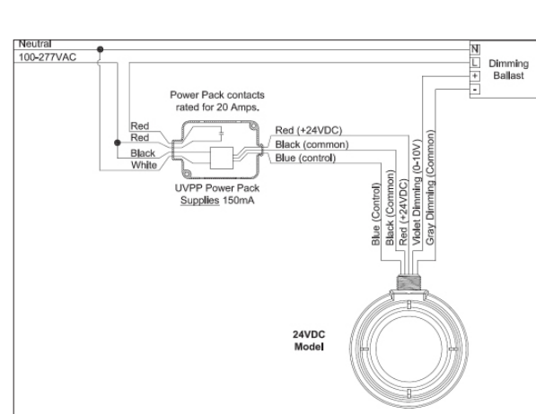
Fig. 5- Wiring Diagram C – Low Voltage Sensor Wiring Diagram
