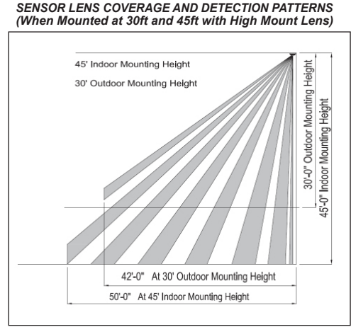
Fig. 7 – Side View of Lens Coverage Pattern at 30ft and 45 ft
