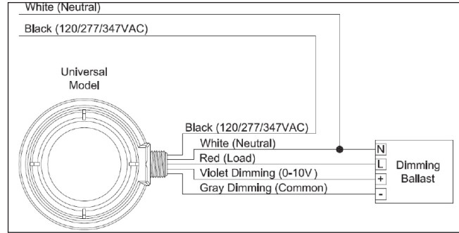
Fig. 3 - Wiring Diagram A – 120/277/347 VAC Line Voltage Wiring Diagram
