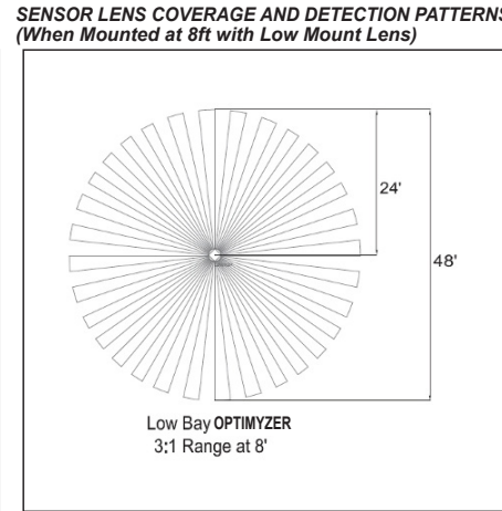
Fig. 6 – Top View of Lens Coverage Pattern at 8 ft
