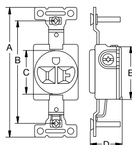
Single Receptacle
