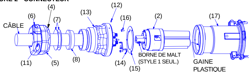
FIGURE 3 • PRISE
