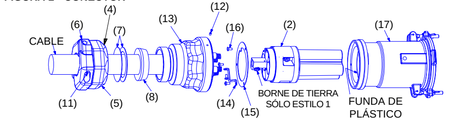
FIGURA 2 • CONECTOR
