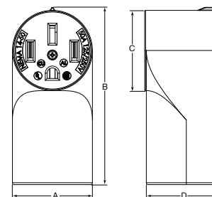
Surface Receptacle
