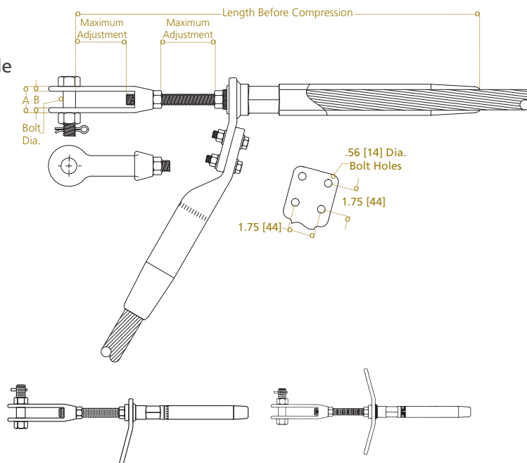
Single Tongue, Adjustable Clevis
