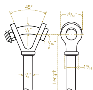
Y-Clevis Ultimate Strength – 50,000 lb FIGURE 8
