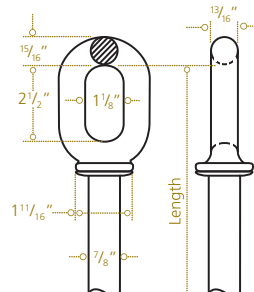
Chain Eye Ultimate Strength – 60,000 lb FIGURE 3
