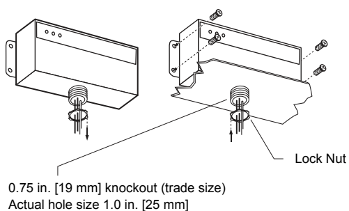
Figure 4: Mounting Unit
