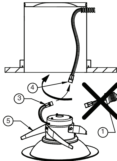
DEDICATED LED HOUSING FOR TITLE 24
