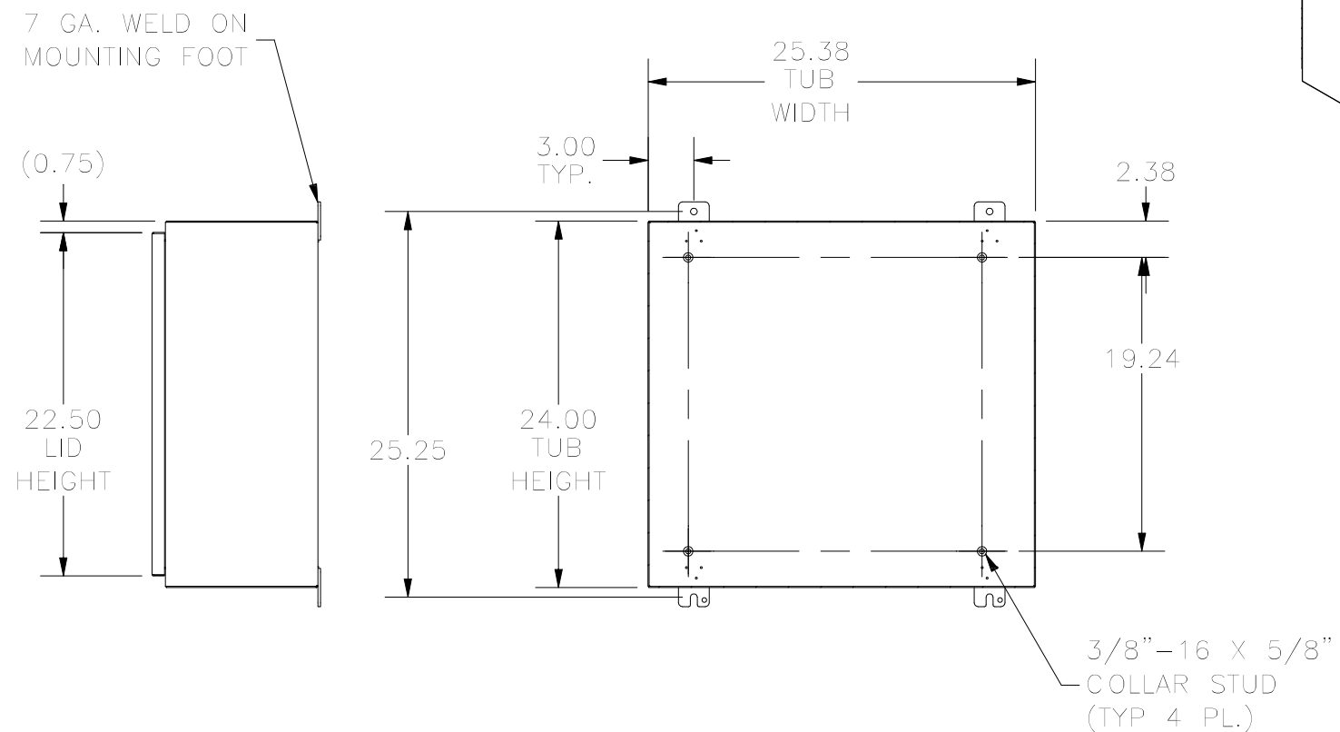
RIGHT VIEW
