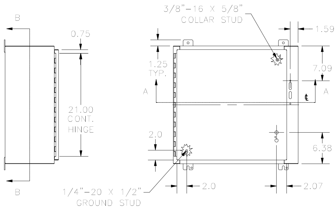
LEFT VIEW
