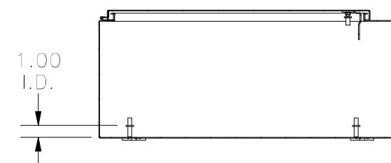
SECTION A-A (INSIDE TOP OF ENCLOSURE)
