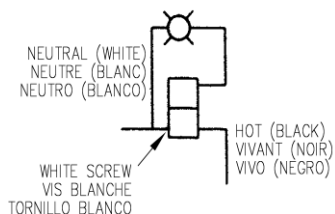
Single Pole Pilot Light Lampe témoin unipolaire Lámpara piloto unipolar
