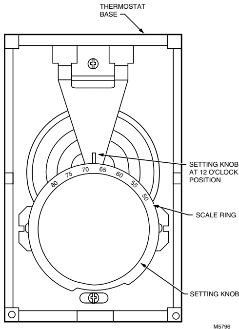
Fig. 5. Calibrating thermostat.
