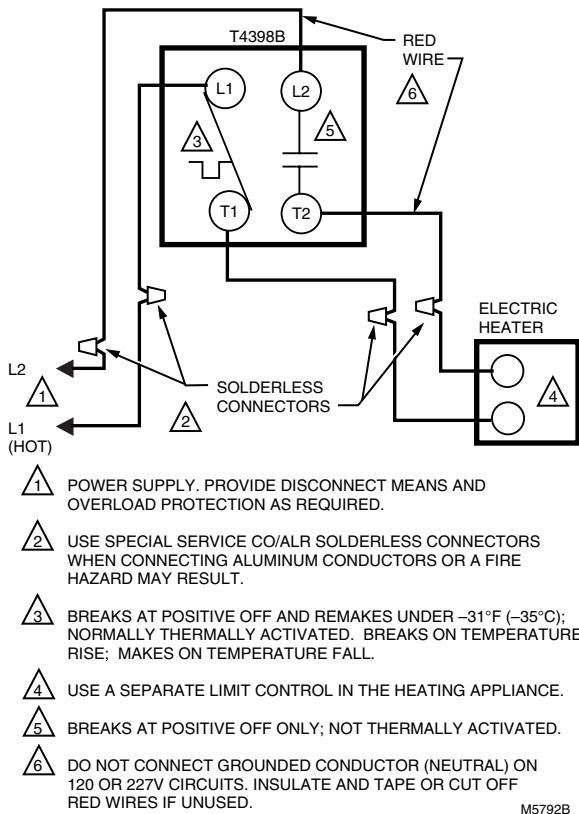
Fig. 3. Typical wiring connections for T4398B.
