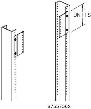
Panel Adapter
