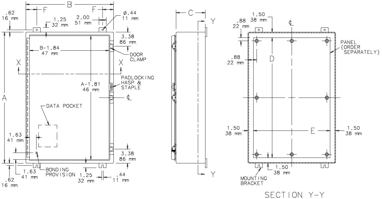
SECTION Y-Y
