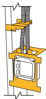
CER4 MC/AC and Non-Metallic Sheathed Cable Support
