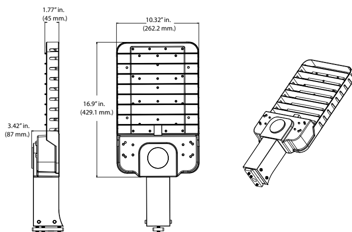
100-140W Model
