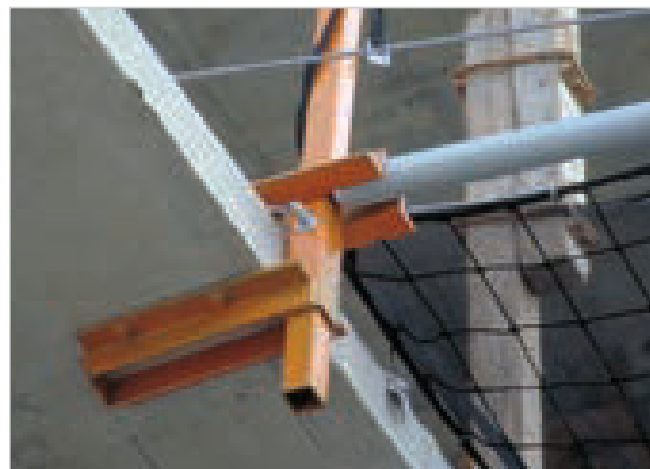
Border Guard Stanchion
