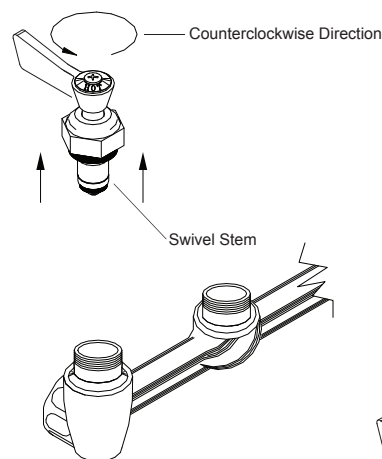
Fig.1 ( Removal of Swivel Stem )
