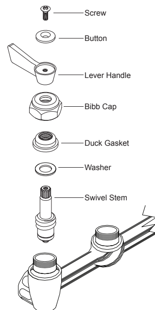
Fig.2 ( Installation of Swivel Stem )
