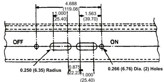
Fig. 3. Flange Drilling Plan for Handle and Interlock Blade Mounting Dimensions.
