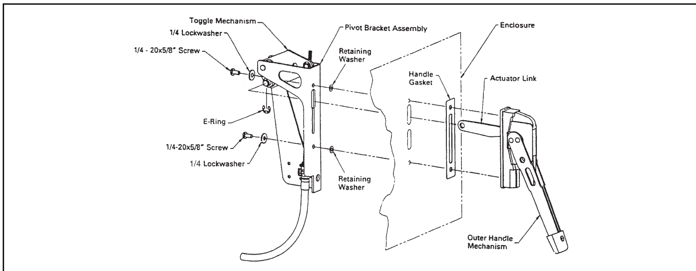
Fig. 1. Pivot Bracket and Outer Handle Mechanism Assembly.
