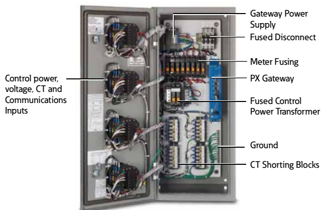
NEMA 12 Single-Unit Enclosed Meter Inside View, PXM 4000/6000/8000 Series
