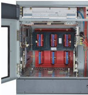
Control Wireway
