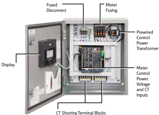
NEMA 12 Single-Unit Enclosed Meter Inside View, PXM 4000/6000/8000 Series
