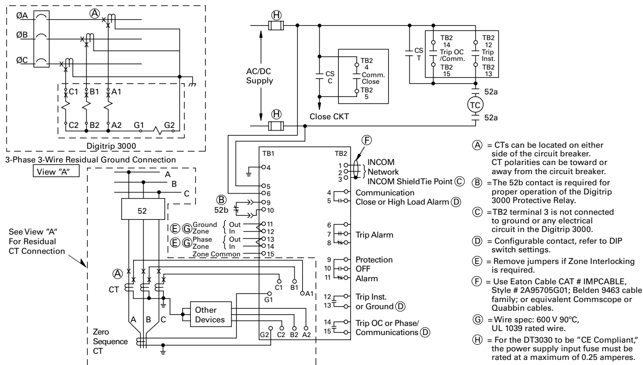
Digitrip 3000 Typical Wiring Diagram
