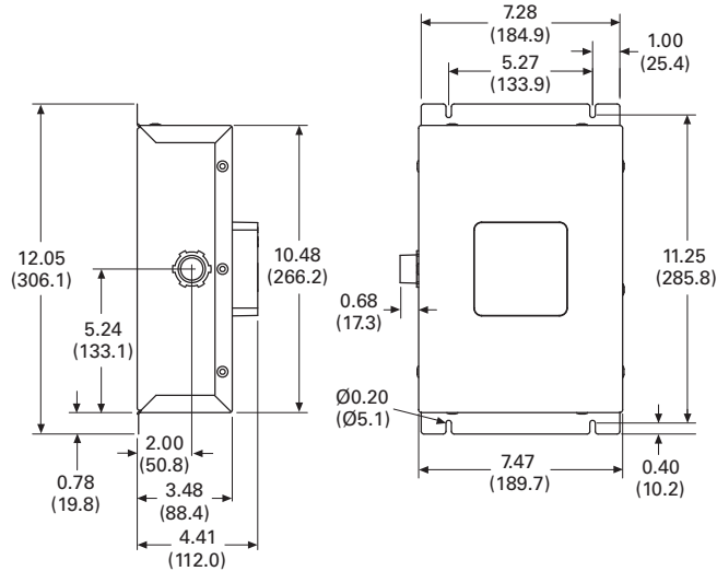
250–400 kA Units in a NEMA 1 Rated Enclosure, Weight = 13.5 Lb
