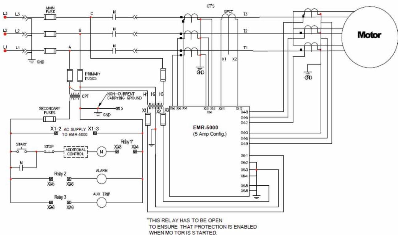
Typical Control Diagram
