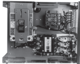
F-10 Unitrol Replacement Starter Unit (1972 to 1989)
