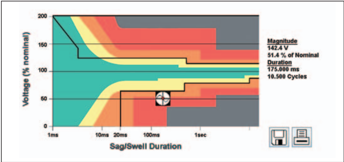
ITIC Curves Sample ITIC curve as displayed by the Power Xpert Meter
