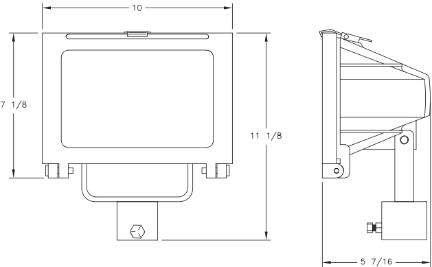
QA-L post mount
