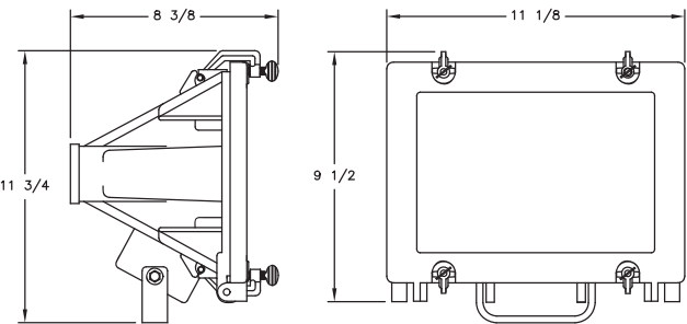
QA-C trunnion mount
