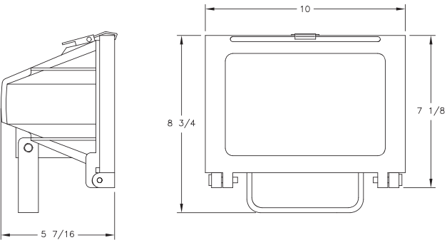
QA-L trunnion mount
