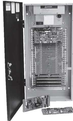
Pow-R-Command Lighting Control
