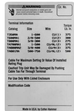
Vintage Label for Typical SELTRONIC Molded-Case Circuit Breaker
