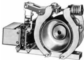
Size 4-Inch Brake and Wheel
