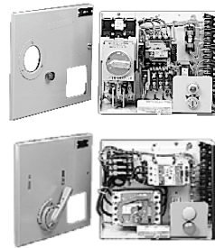
Motor Control Center Bucket Retrofits
