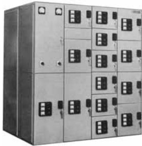
Pow-R-Gear Switchboard, St. Louis Vintage with Drawout SPB Breakers
