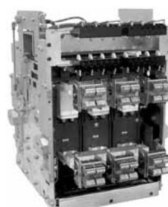
DB25-AR600NM—Rear View
