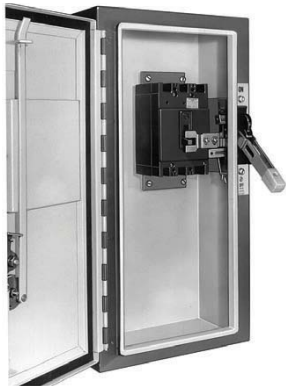
Enclosed Breaker with SM Handle
