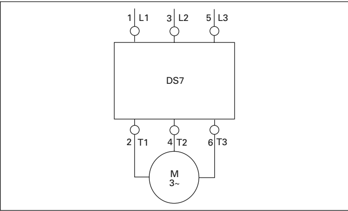
Figure 2. Power wiring diagram
