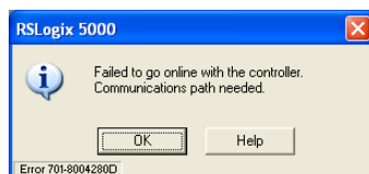
Figure 61: Error message
