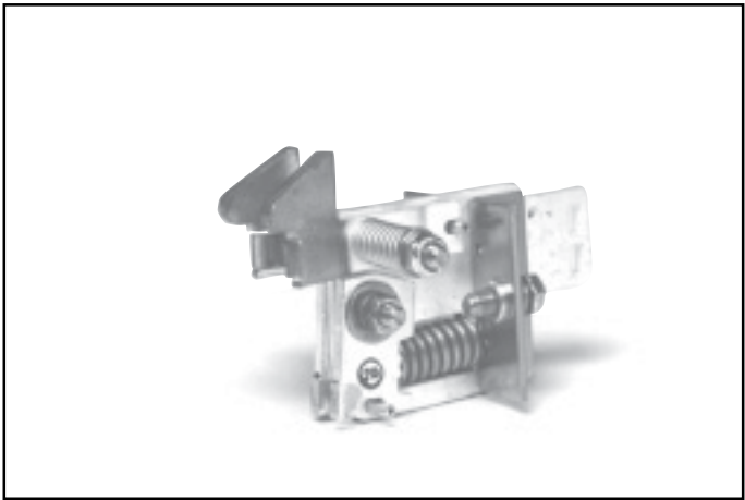
Figure 4.4 DS-206 Upper Stud Assembly
