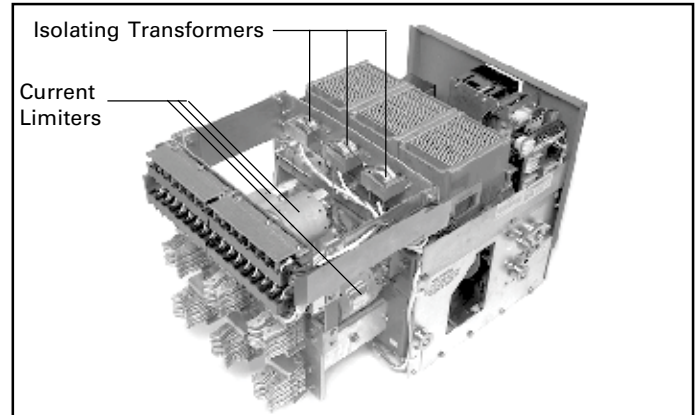
Figure 21.2 DSL-416 w/o barriers
