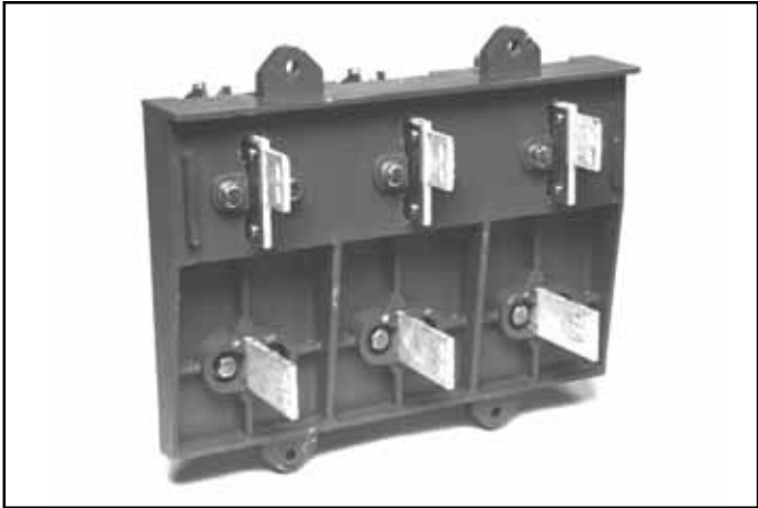
Figure 4.2 DS-206 Pole Unit Assembly Rear View
