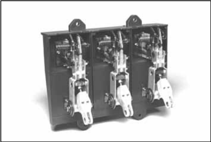
Figure 4.1 DS-206 Pole Unit Assembly Front View
