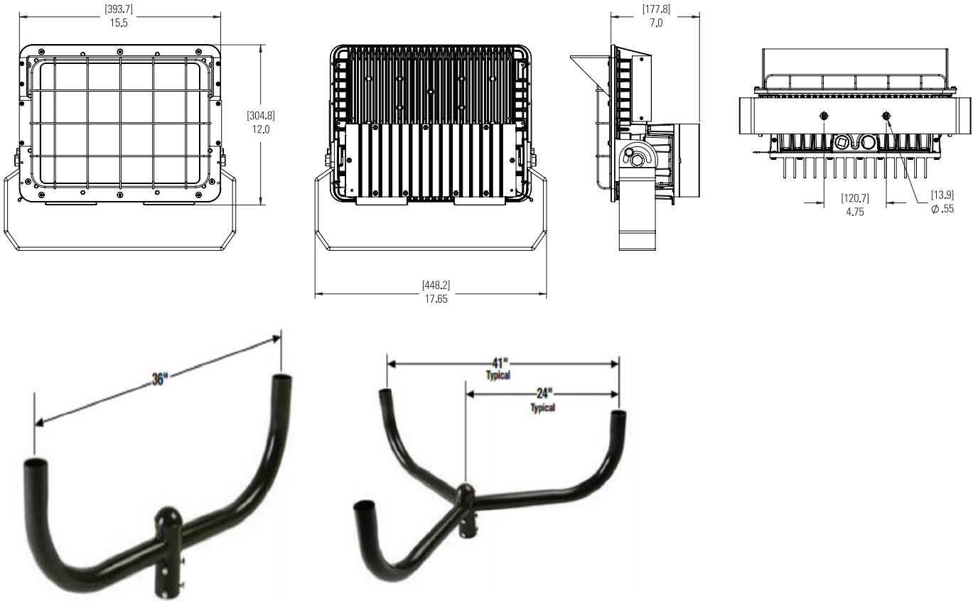
Bull horns – provided with 2 3/8" pole tenon
