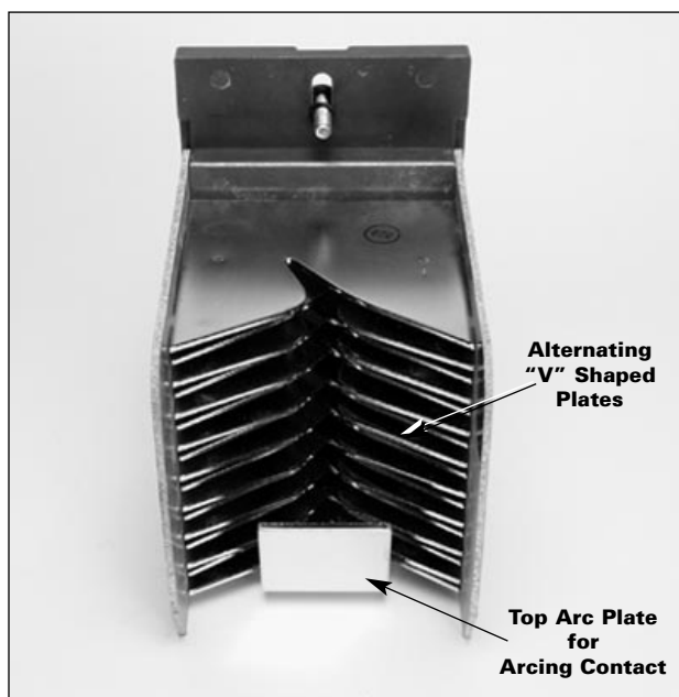
Arc Chute (Bottom View)
