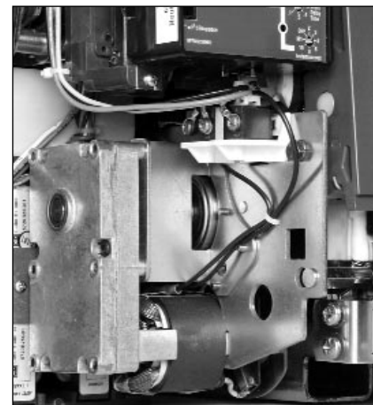
Figure 10 Motor Operator Installed in Narrow Frame Circuit Breaker
