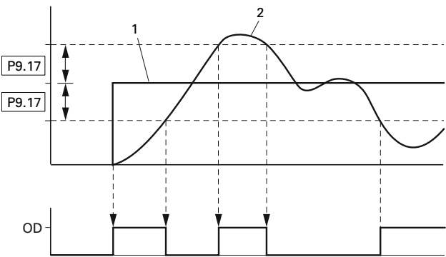
Function Chart for OD (PID System Deviation)
