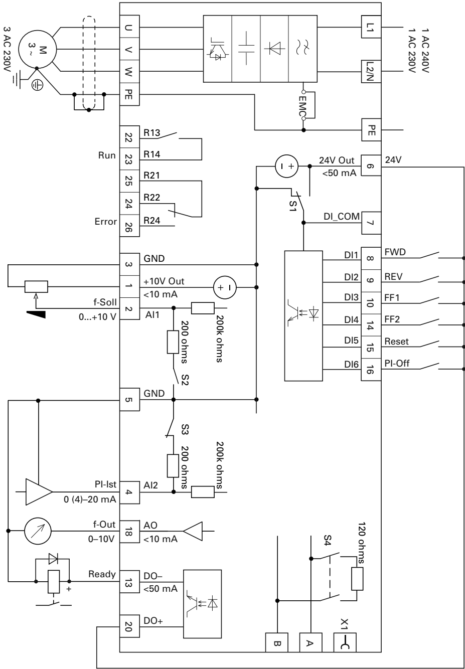
MMX12...F Block Diagram
