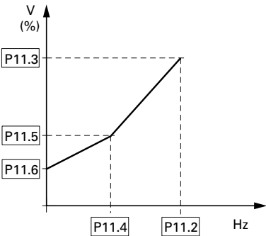
Configurable P11.1 = 2
