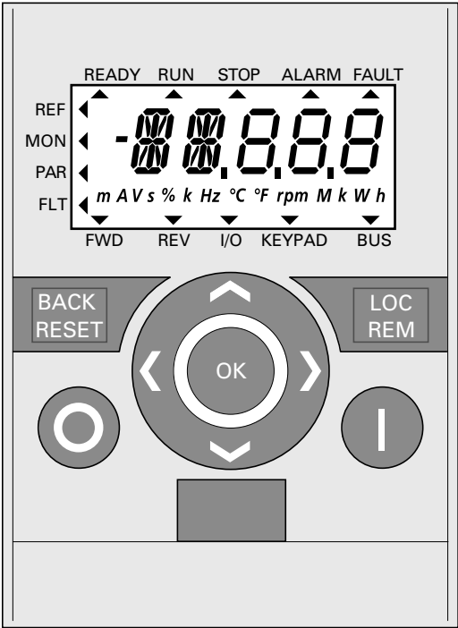
View of the Keypad with LCD Display, Function Keys and Interface (LCD = Liquid Crystal Display)
