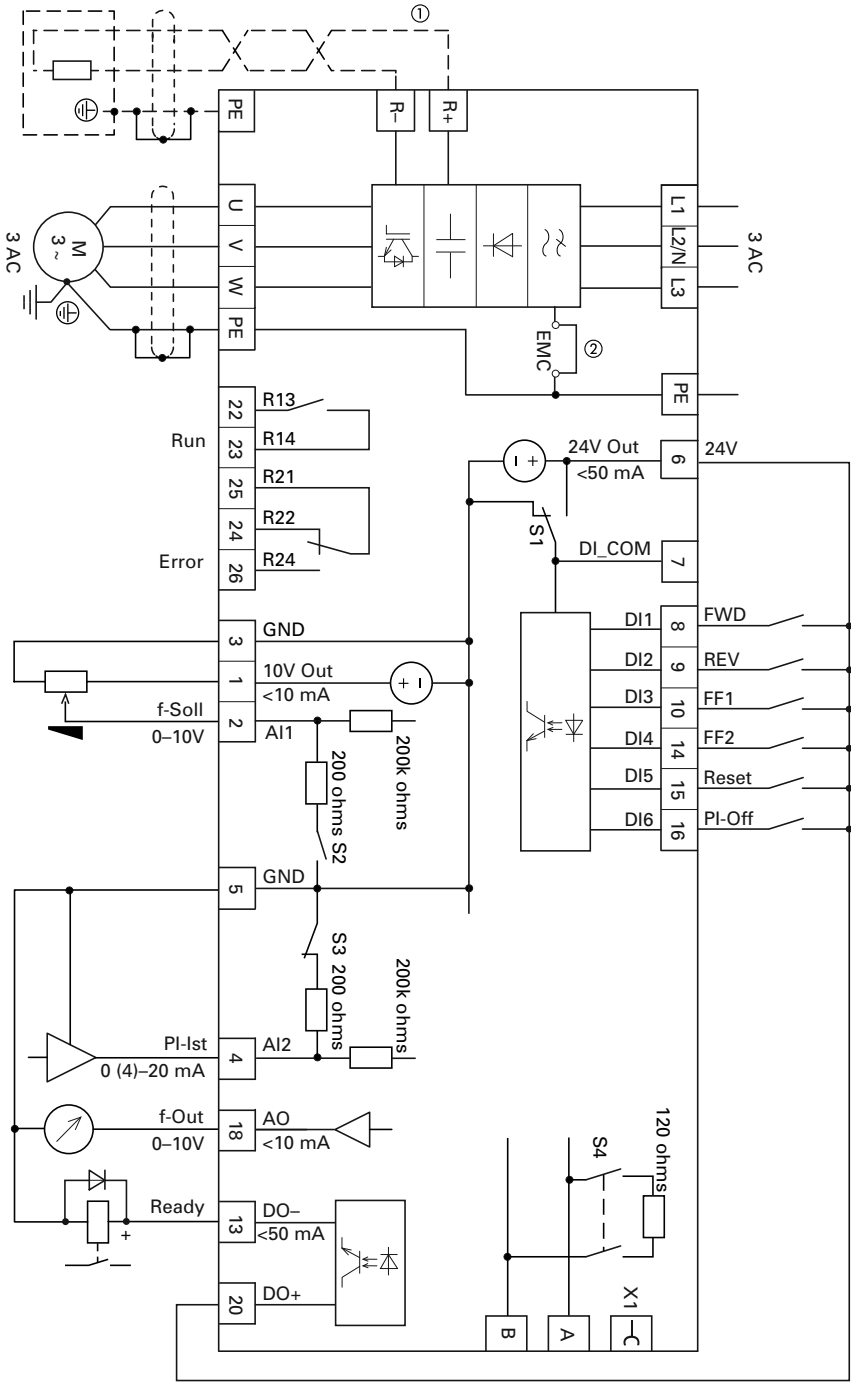
MMX32, MMX34 and MMX35 Block Diagram
