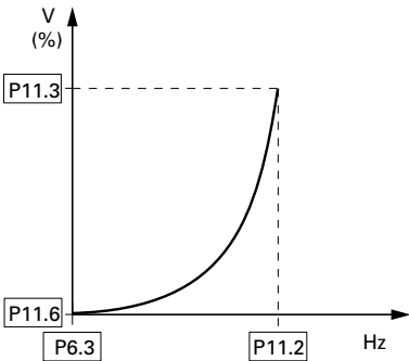
Squared P11.1 = 1
