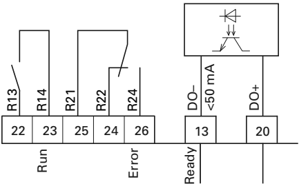
Digital Outputs
