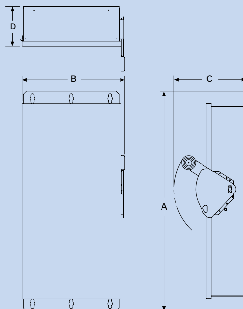
NEMA Type 4, 4X stainless dimensions
