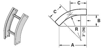
45° Vertical Outside
