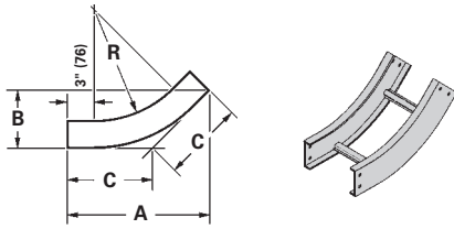
45° Vertical Inside
