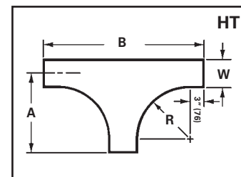
Horizontal Tee Ventilated Horizontal Tee
