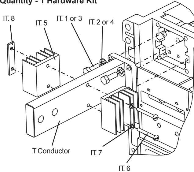
PDG6 Rear Conductor Hardware Kit Quantities
