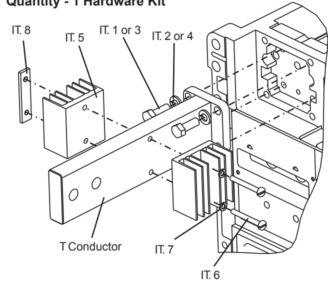
PDG6 Rear Conductor Hardware Kit Quantities
