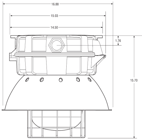
Ceiling mount
