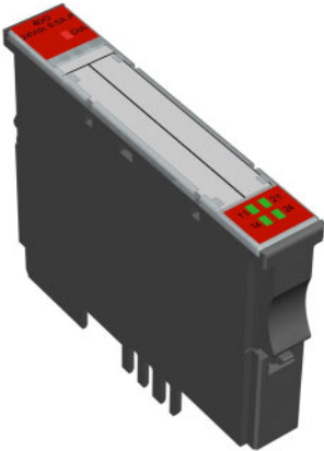
Figure 100: Digitale output module, 4 digital outputs, 24 V DC, 2 A, positive switching
