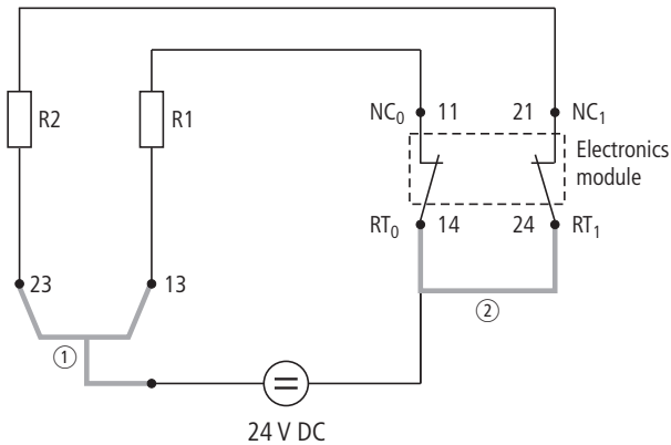
Figure 127: Module circuit diagram XN-S4x-SBCS
