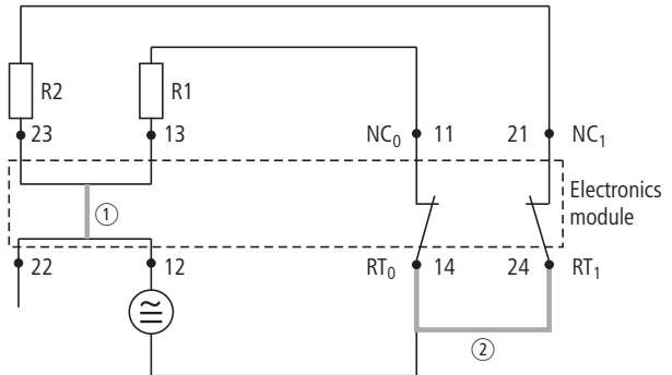
Figure 125: Module circuit diagram XN-S4x-SBBS
