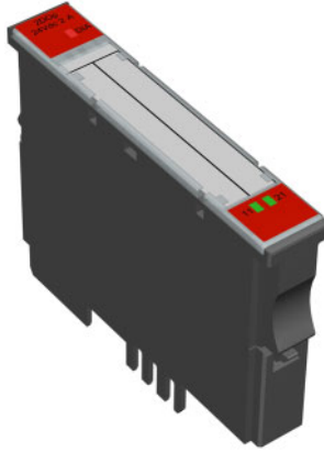
Figure 90: Digitale output module, 2 digital outputs, 24 V DC, 2 A, positive switching
