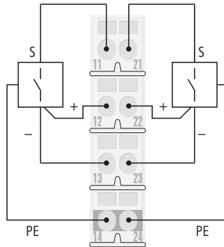
Figure 47: Connection diagram XN-S4x-SBBC
