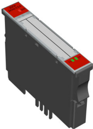
Figure 85: Digitale output module, 2 digital outputs, 24 V DC, 0.5 A, negative switching
