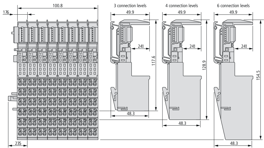
Figure 11: Base module in block design with screw connection (XN-BxS...)
