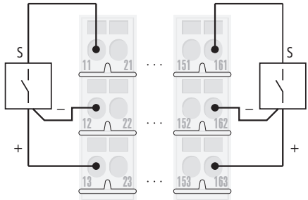
Figure 66: Connection diagram XN-B3x-SBB
