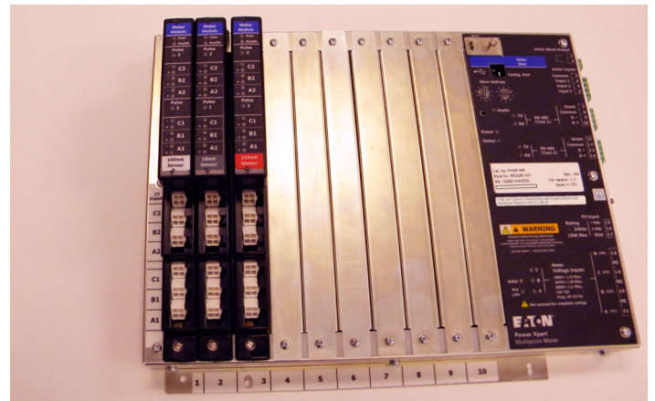
Figure 5. PXMP-MB Assembly Components and LEDs.
