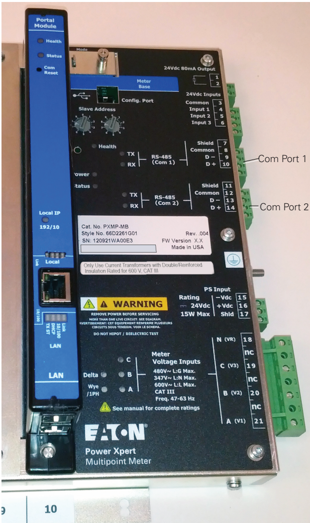
Figure 26. PXMP Communication Ports.
