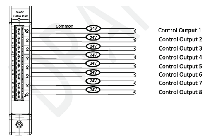
Figure 23. PXMP-DOM Wiring.
