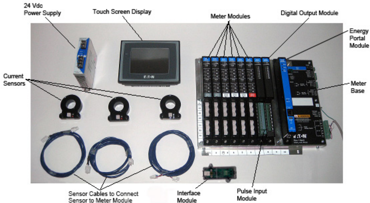
Figure 1. Components of the PXMP Meter System.
