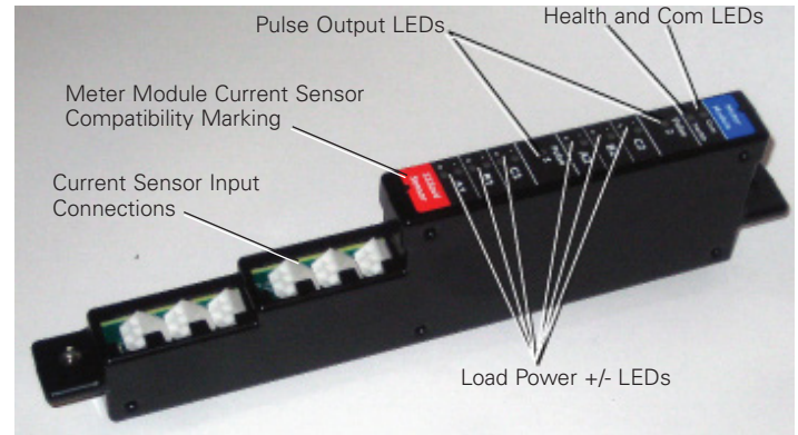
Figure 9. Typical PXMP-MM.
