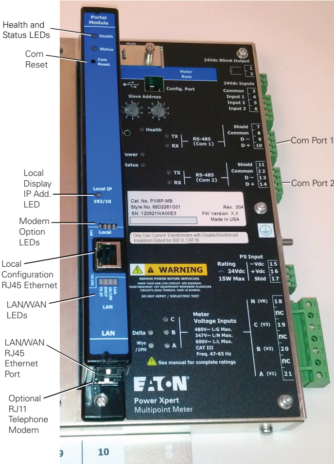
Figure 24. PXMP-EPM.
