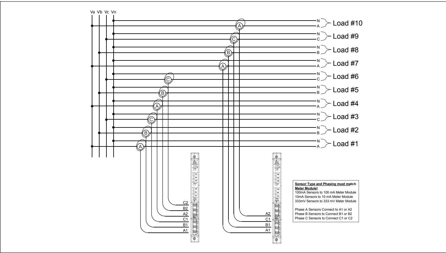
Figure 19. 3-Phase 4-Wire Service Using Ten Single-Phase, 1 Pole Current Sensors.
