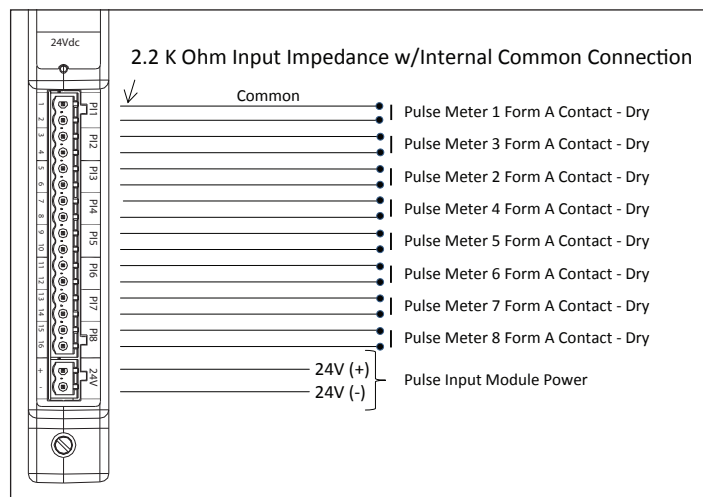
Figure 21. PXMP-PIM Wiring.
