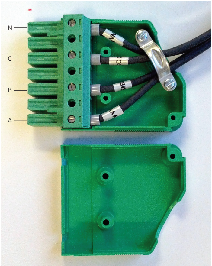
Figure 7. Meter Voltage Input Terminal Plug and Cover.
