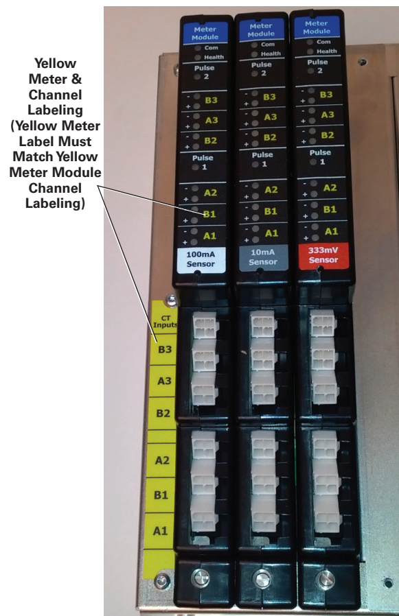
Figure 10. .PXMP-MB-AB Examples.
