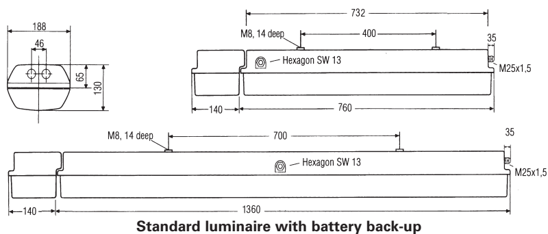
Standard luminaire with battery back-up
