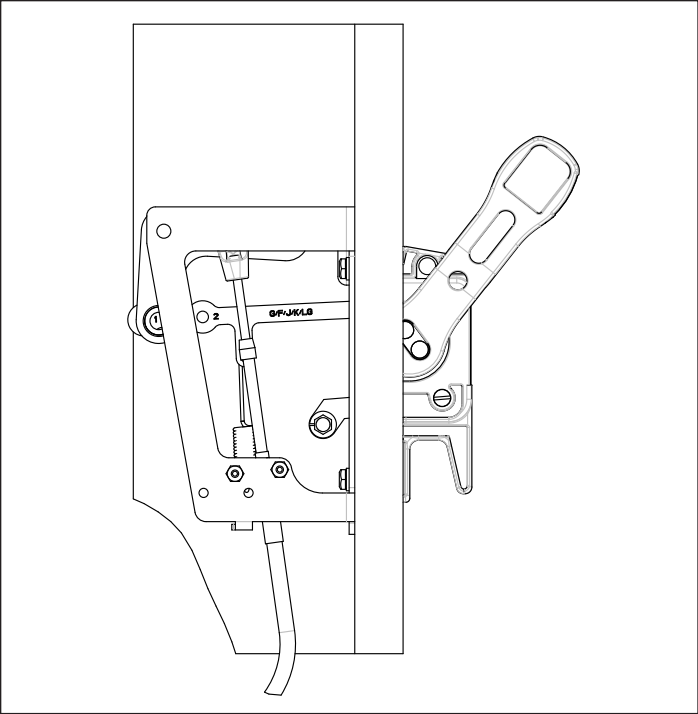
Figure 6. Assembly of spring to toggle mechanism.
