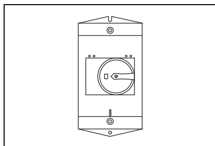
Figure 30.1-15. Frame B (0.1–32 A) XTPR Rotary Manual Motor Protectors H x W x D 6.30 x 3.94 x 5.12 (160.0 x 100.0 x 130.0)
