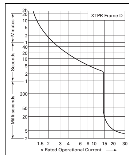
Figure 30.1-21. XTPR Frame D
