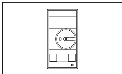
Figure 30.1-16. Frame B (0.1–32 A) XTPR Rotary Manual Motor Protectors with XTPAXFAEM20 Early-Make Front-Mount Auxiliary Contact H x W x D 6.30 x 3.94 x 5.12 (160.0 x 100.0 x 130.0)
