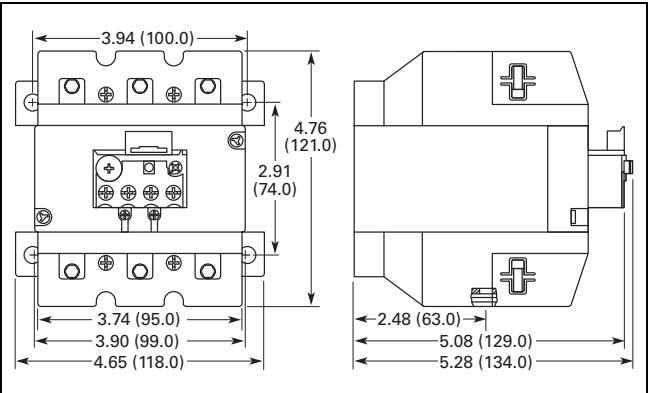
Figure 30.3-16. Frames F–G, XT0B...G1CS Overload Relay
