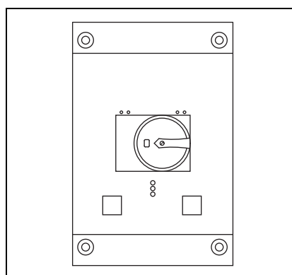
Figure 30.1-19. Frame D (10–65 A) Rotary Motor Protective Circuit Breakers H x W x D 9.45 x 6.30 x 7.76 (240.0 x 160.0 x 197.0)
