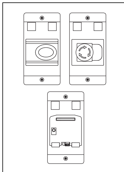
Figure 30.1-18. XTPB Pushbutton Manual Motor Protectors H x W x D 6.22 x 3.15 x 4.59 (158.0 x 80.0 x 116.5)
