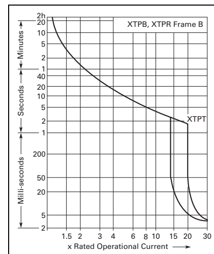
Figure 30.1-20. XTPB, XTPR Frame B
