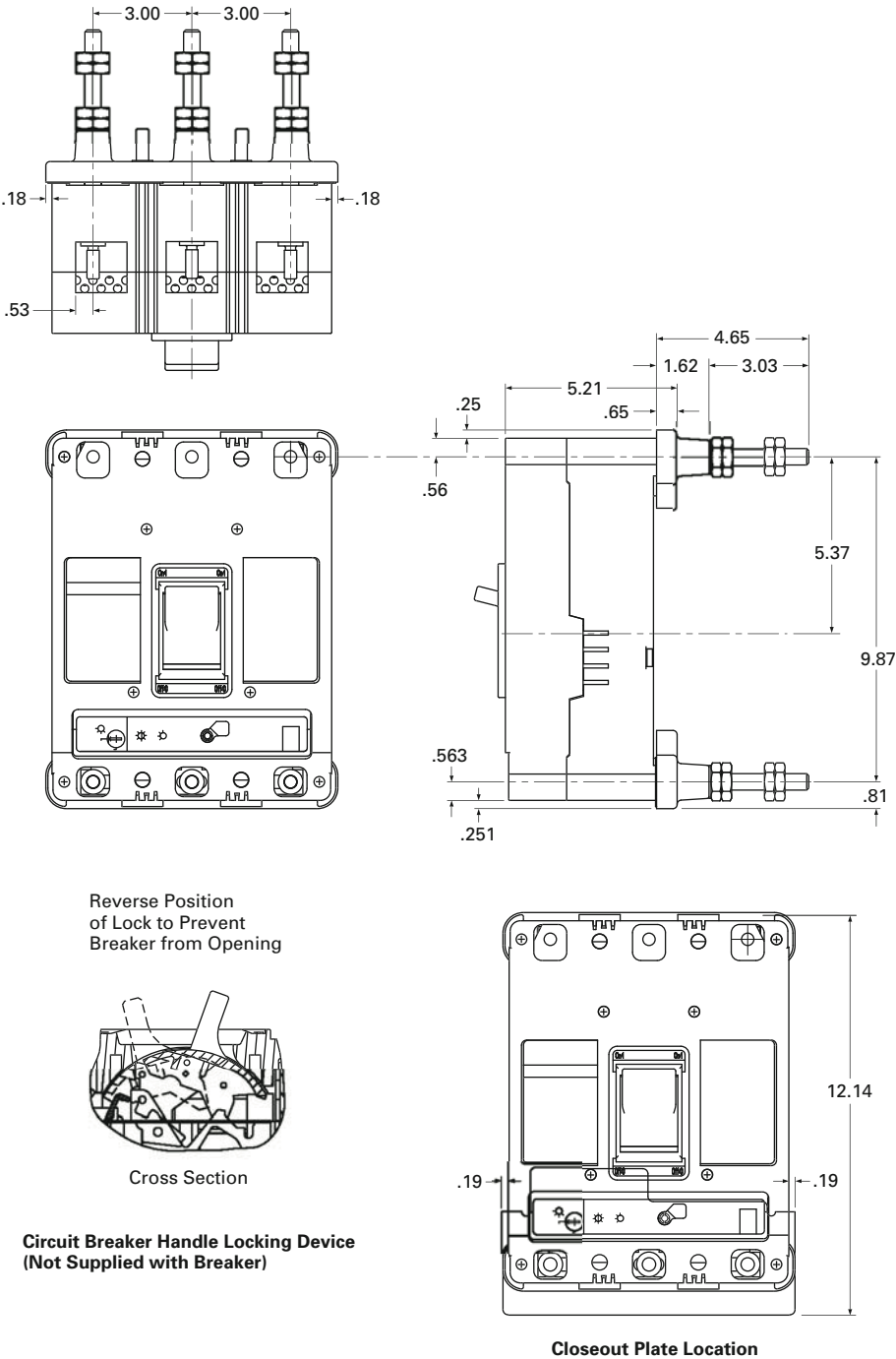
Outline Dimensions AQB-A253, AQB-L253 and NQB-A253 Breakers — Dimensions in Inches
