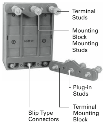
Rear view of breaker showing terminal blocks for switchboard mounting. (Terminal block attached at line end of breaker and removed from load end.)
