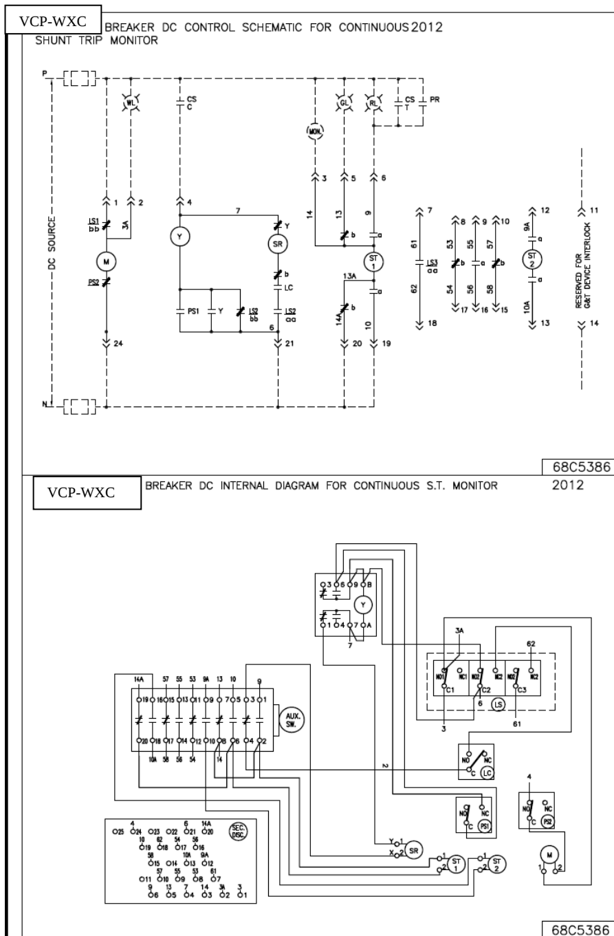
Figure 5-5A 15kV VCP-WXC 63kA 1200-3000A Special Power Plant Breakers, Styles: 4A35390G10, 4A35391G10, 4A35392G10 - DC Control Scheme and Diagram
