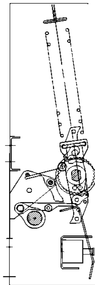
Breaker Closed, Springs Charged
