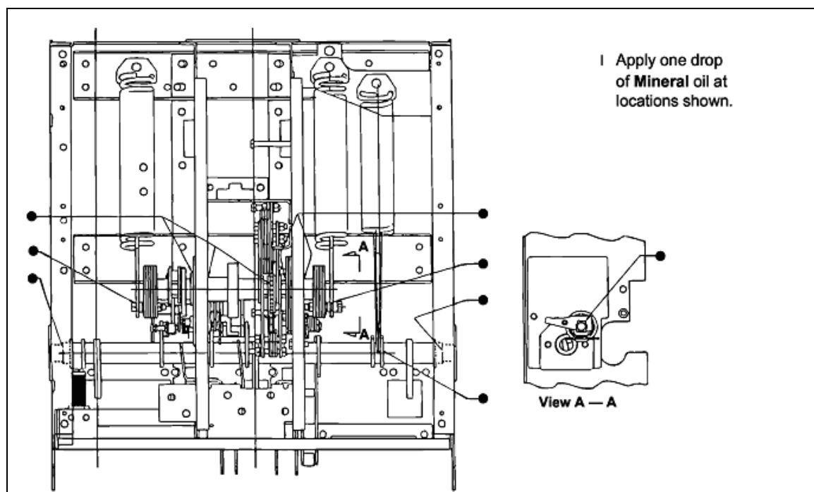
Figure 6-1 lubrication points
