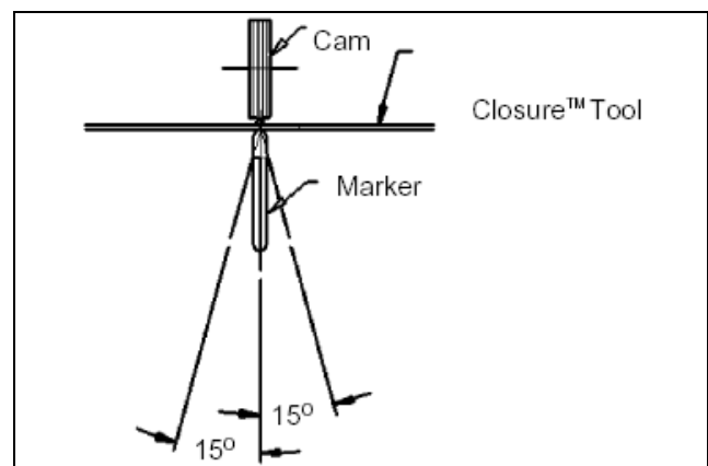
Figure 6-13 Top View of Cam and Marker interface
