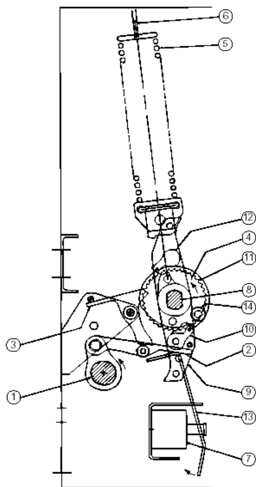
Breaker Open, Springs Discharged
