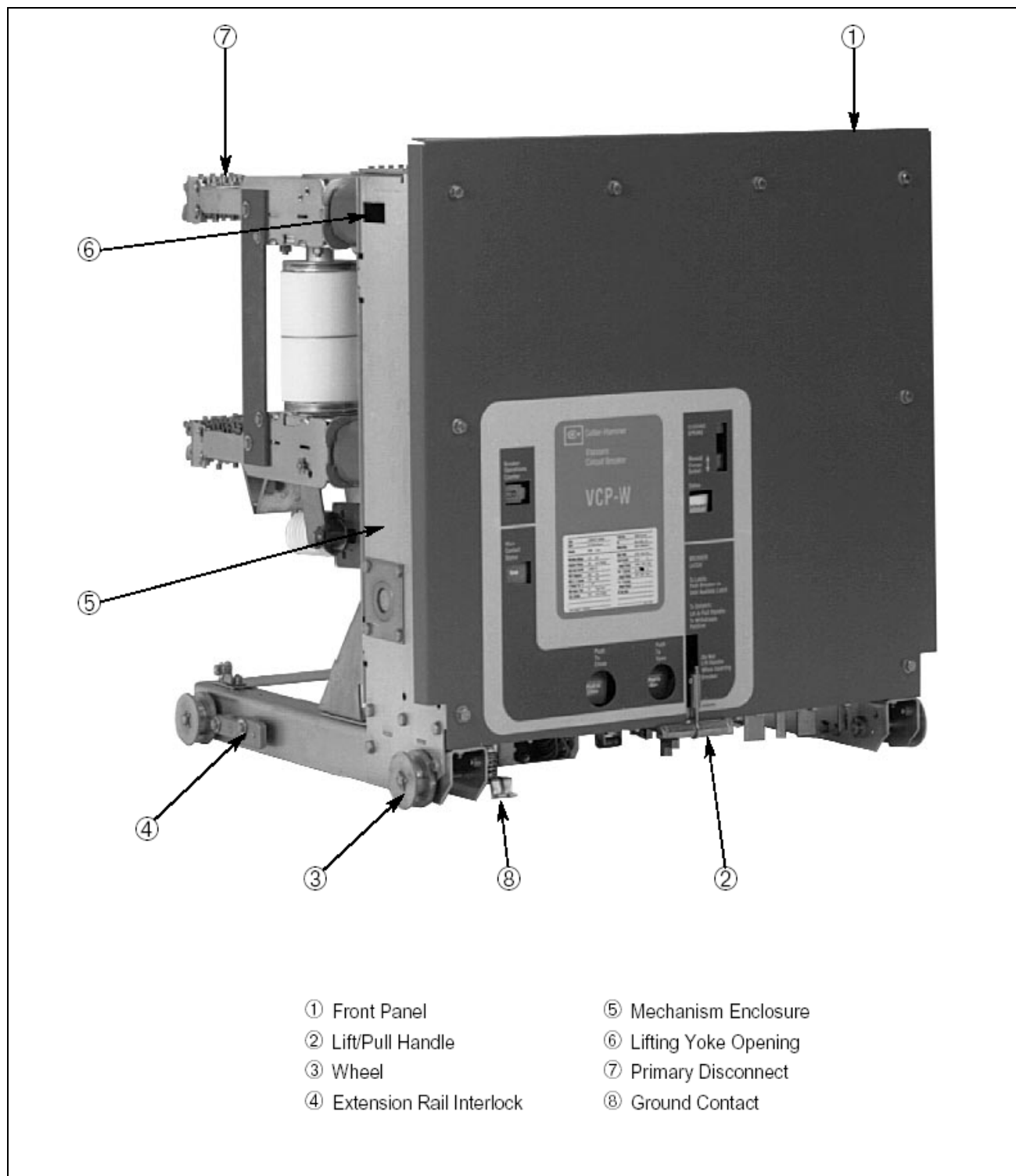
Figure 3-2 Typical Front View VCP-W Vacuum Circuit Breaker (Newer model Breakers may not have the escutcheon as shown)
