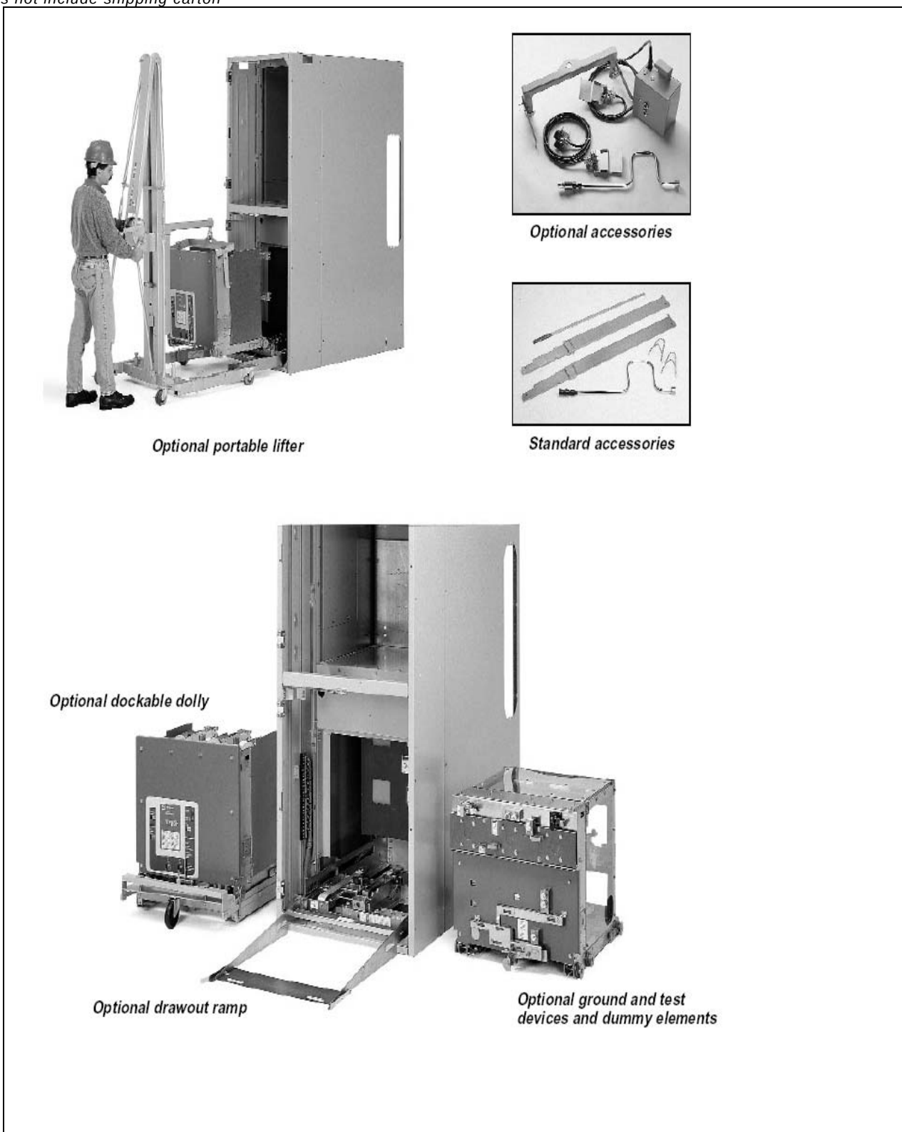
Figure 3-1 Typical VCP-W Tools and Accessories (Note: Products shown for representation only. New products may include design improvements and alternate nameplate configurations.)
