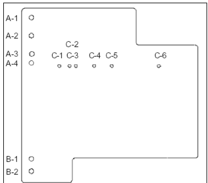
Figure 6-19 Front view of closure tool showing Mounting/testing locations (6352C49H01)
