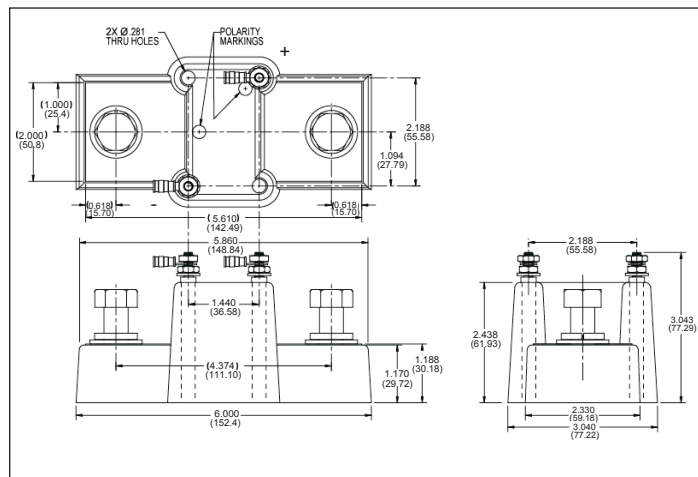
Figure 9. Neutral Sensor Dimensions (CTF080, CTF160, and CTF225).
