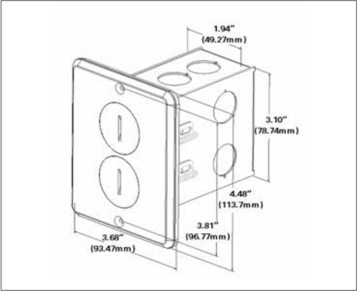
Figure 2. TR5249B Series
