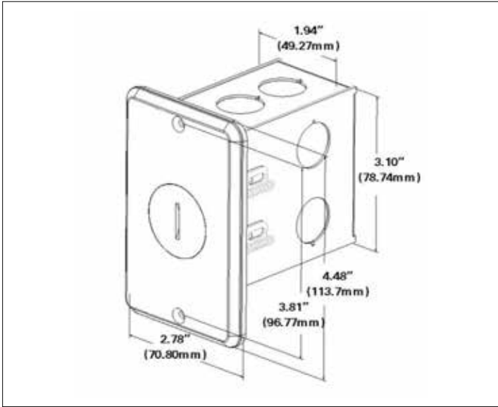
Figure 1. TR5797 Series
