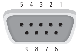
Figure 24: 9-pin SUB-D socket on connecting cable to PC (top view)
