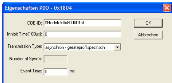
Figure 39: PDO properties (Send PDO mapping)
