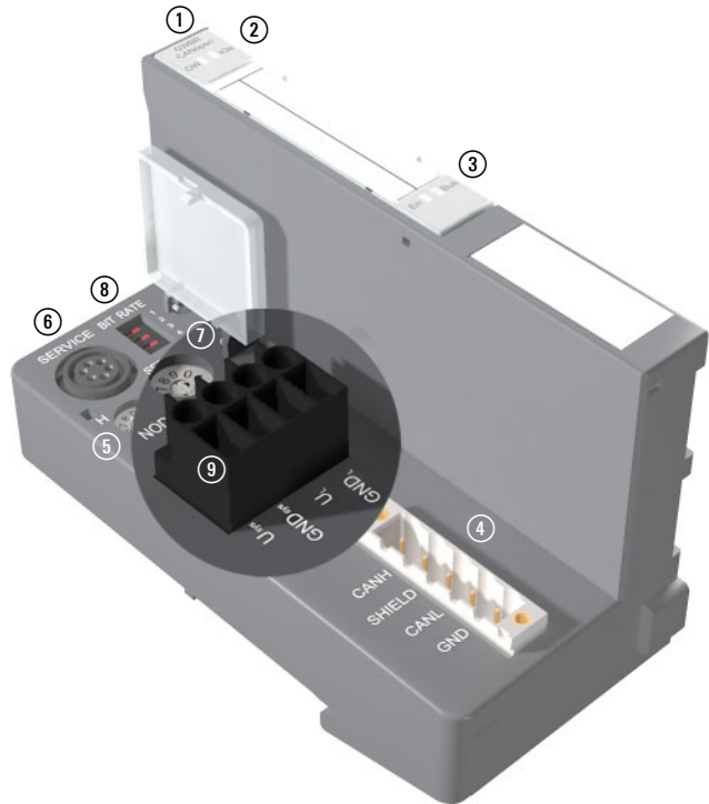
Figure 3: XN-GWBR-CANopen
