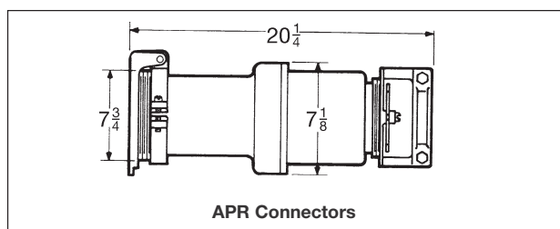
AP Plugs
